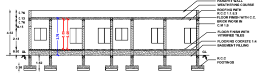
SECTION ON "S S"
