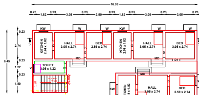
PROPOSED GROUND FLOOR PLAN
