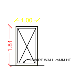
WICKET GATE
