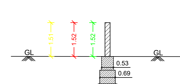
COMPOUND WALL
