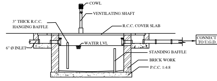
SECTION DETAILS OF SEPTIC TANK
