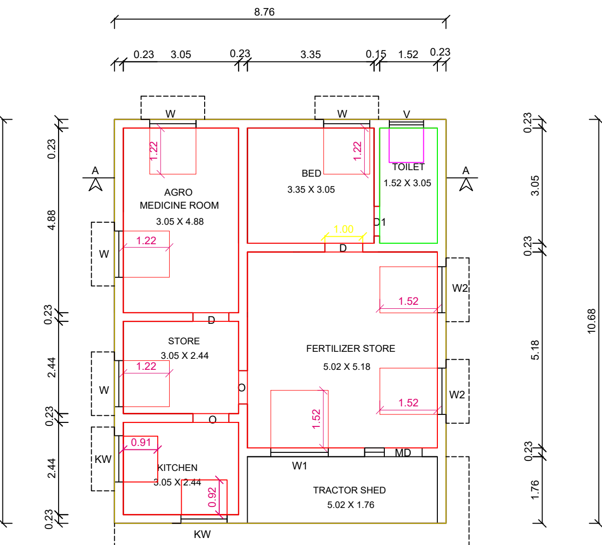
FARM HOUSE PLAN
