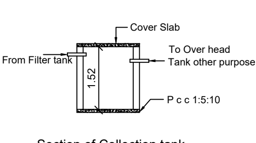
Section of Collection tank
