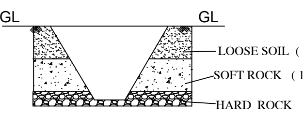
TRIAL PIT
