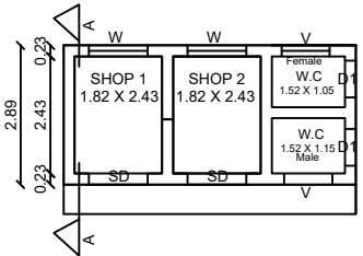
ADDITIONAL SHOP BUILDING GROUND FLOOR PLAN
