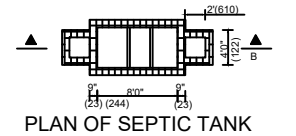
PLAN OF SEPTIC TANK
