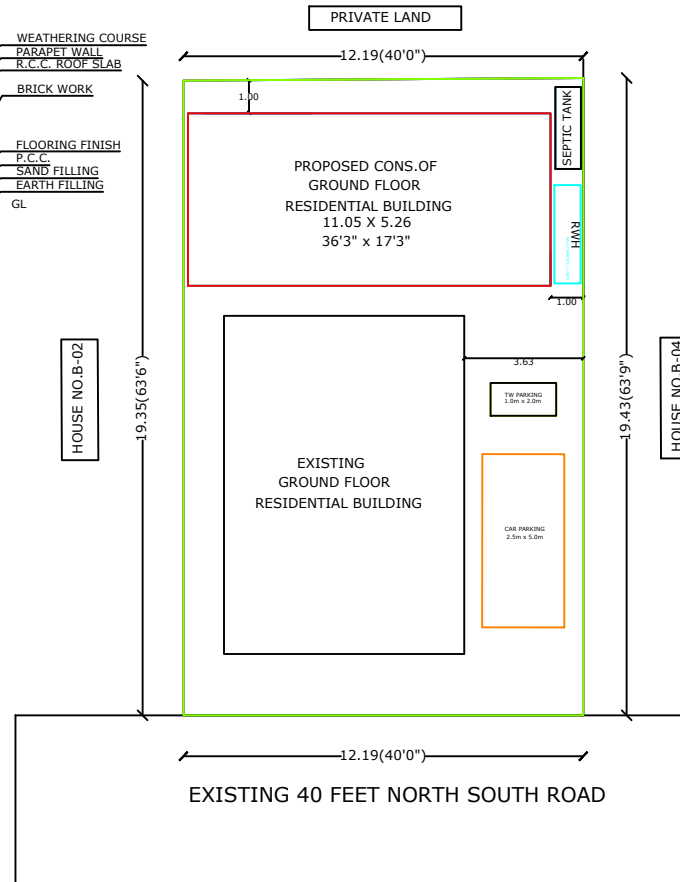
SITE PLAN
