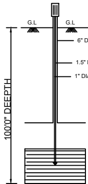
BORE WELL
