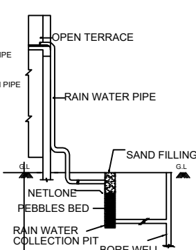
RAIN WATER
