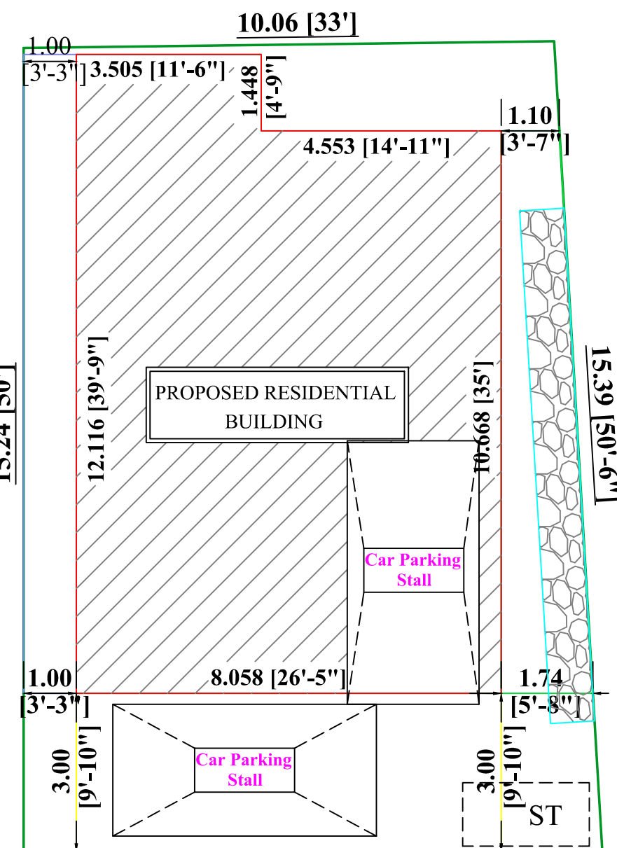
22' WIDE EAST WEST LAYOUT ROAD
