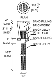
RAIN WATER HARVESTING PERCOLATION PITS
