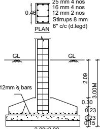
COLUMN DETAILS
