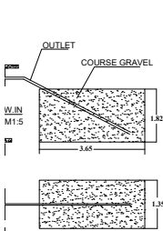
SEPTIC TANK & D-TRENCH DETAILS
