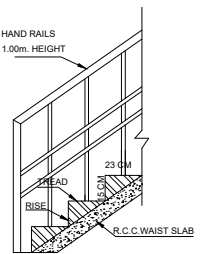
SECTION ON STAIRCASE
