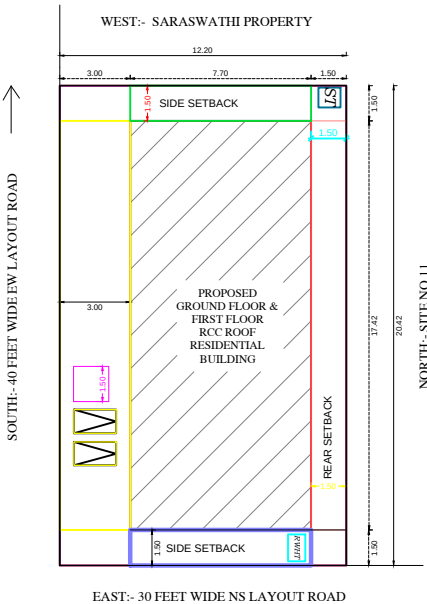
SITE PLAN
