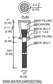
RAIN WATER HARVESTING PERCOLATION PITS
