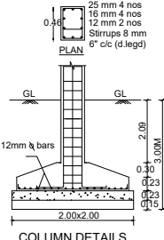
COLUMN DETAILS
