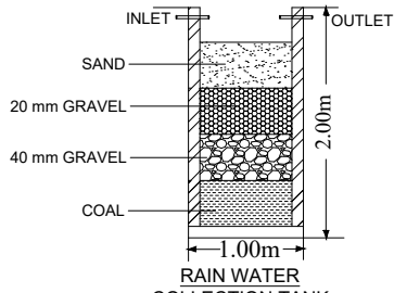
RAIN WATER COLLECTION TANK
