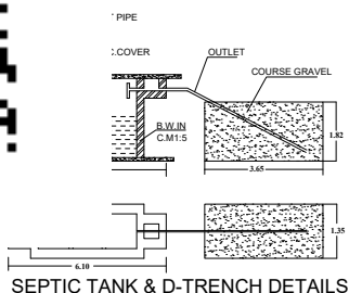
SEPTIC TANK & D-TRENCH DETAILS
