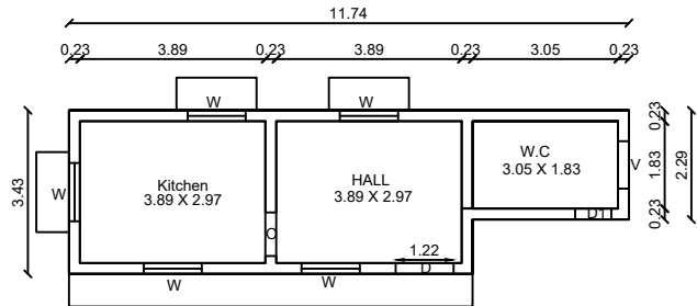
FARM HOUSE GROUND FLOOR PLAN
