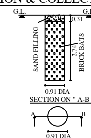
DETAILED PLAN OF RAINWATER PERCOLATION & COLLECTION PIT
