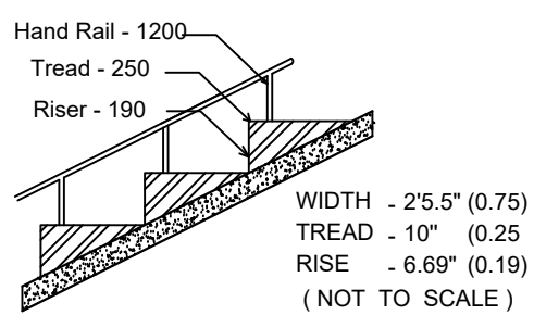
STAIRCASE DETAILS
