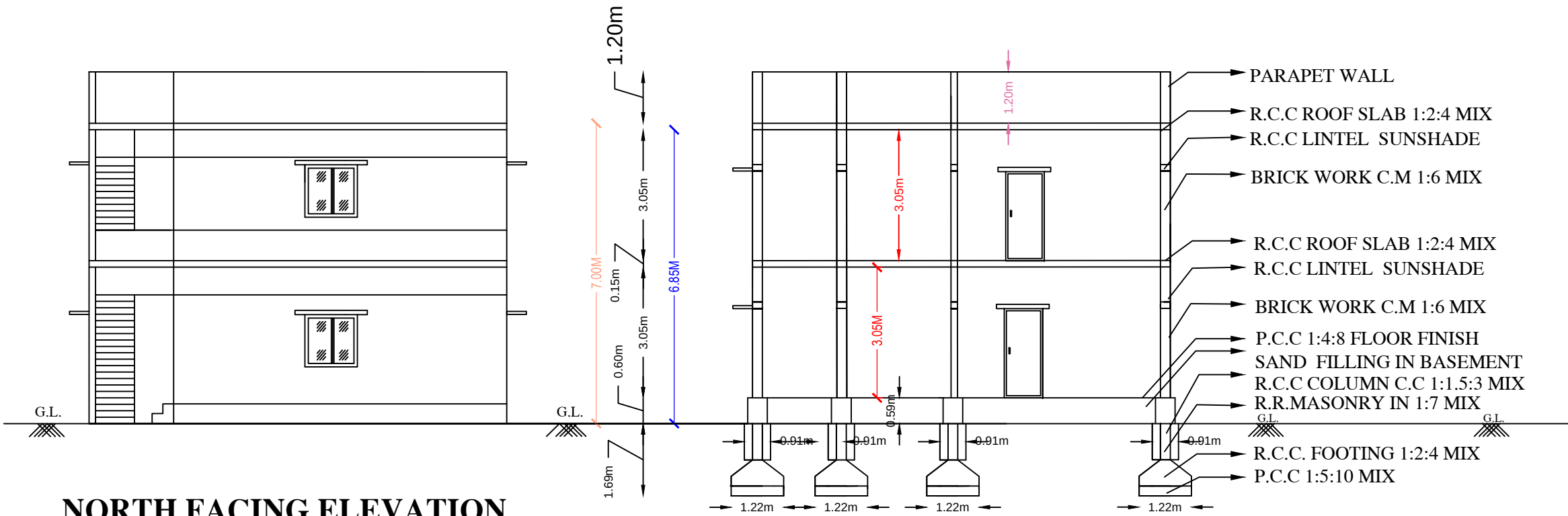
NORTH FACING ELEVATION
