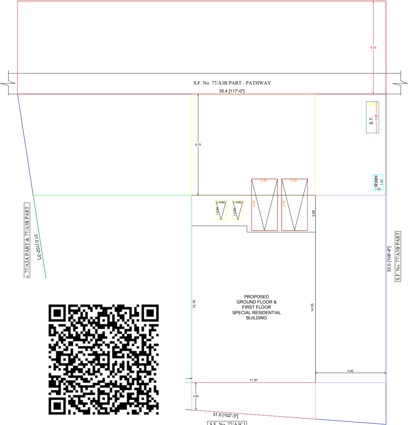
SITE PLAN
