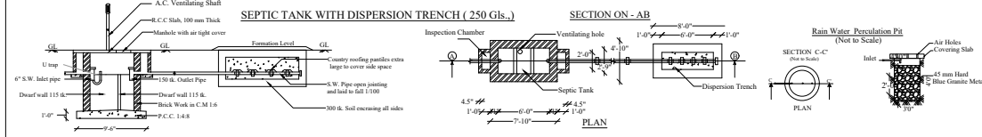
SEPTIC TANK WITH DISPERSION TRENCH (250 Gls.)
