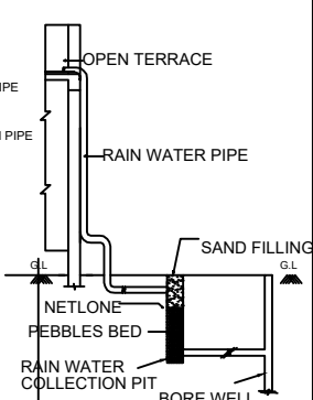
RAIN WATER
