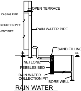
RAIN WATER
