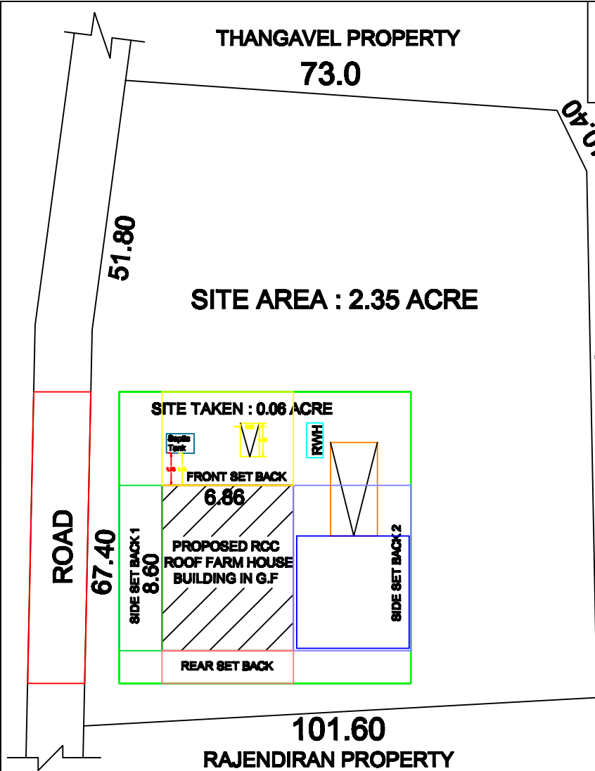
SITE PLAN-NOT TO SCALE
