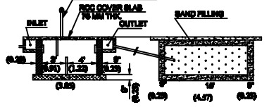
SECTION ON SEPTIC TANK & DISP-TRENCH
