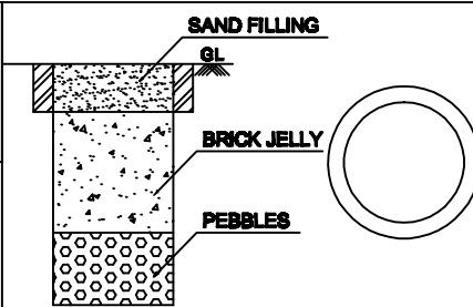
RAIN WATER HARVESTING SYSYTEM
