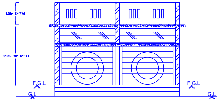
ELEVATION WEST FACING
