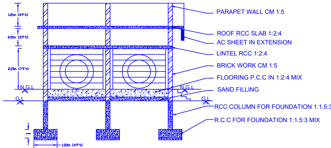
SECTION ON-AA
