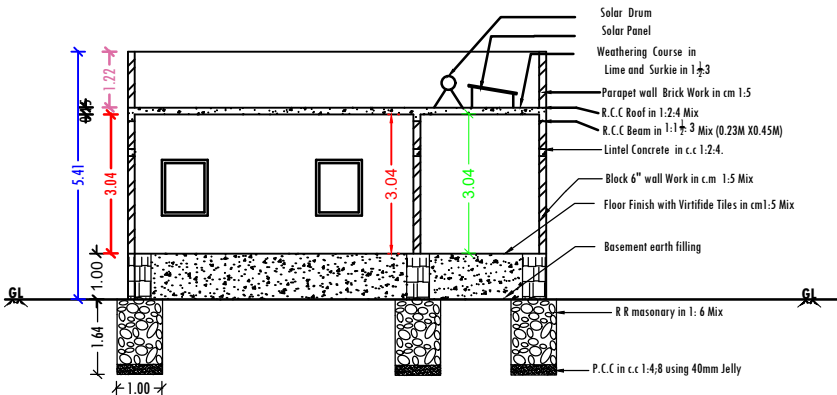
Section on "BC"
