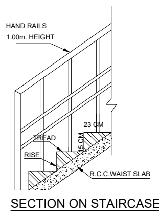
SECTION ON STAIRCASE
