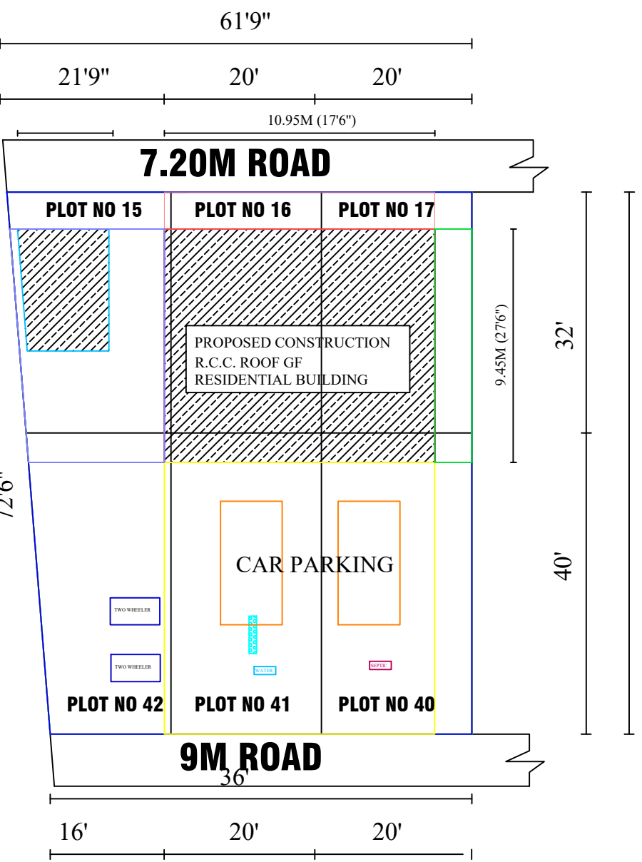
SITE PLAN
