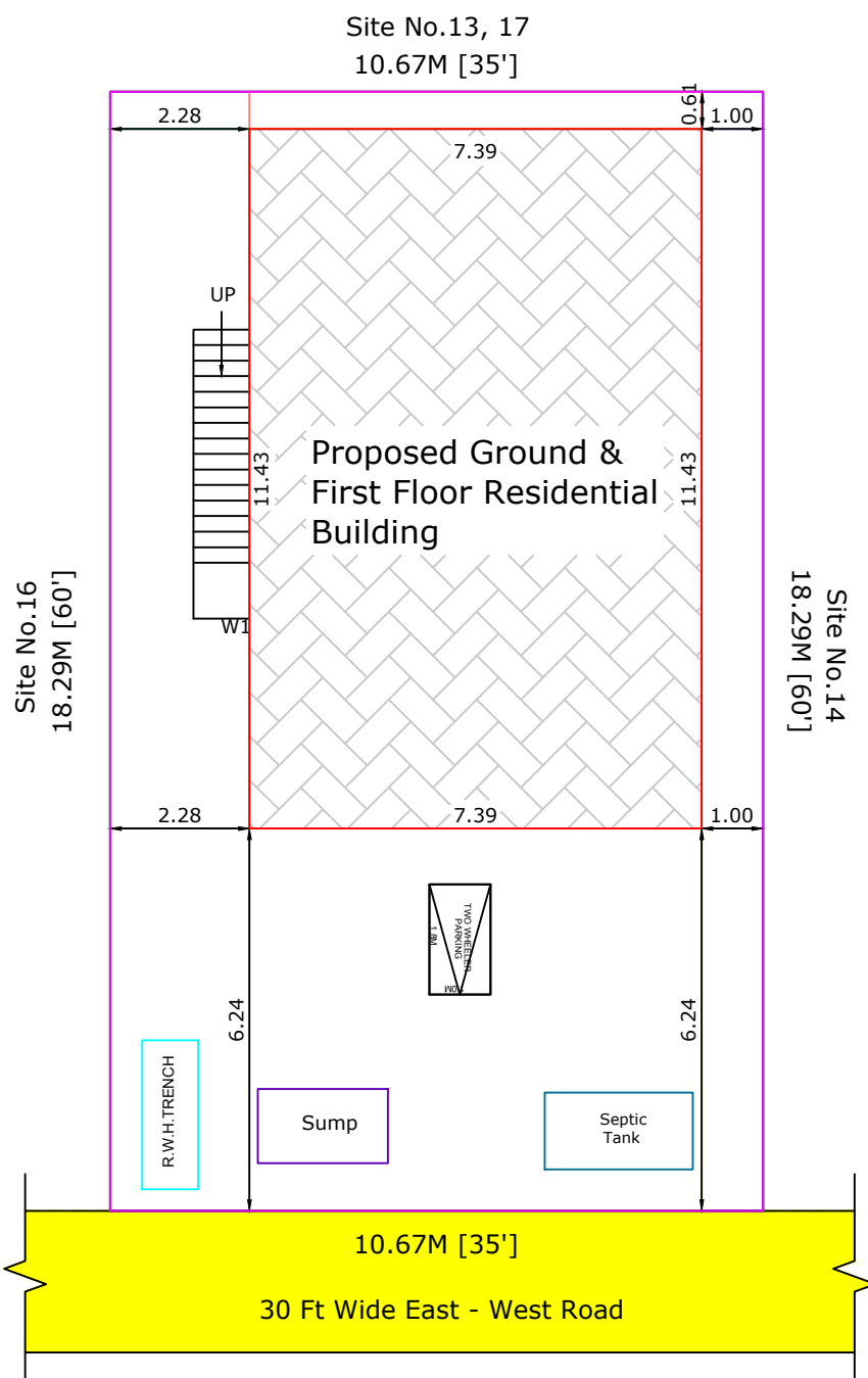
SITE PLAN
