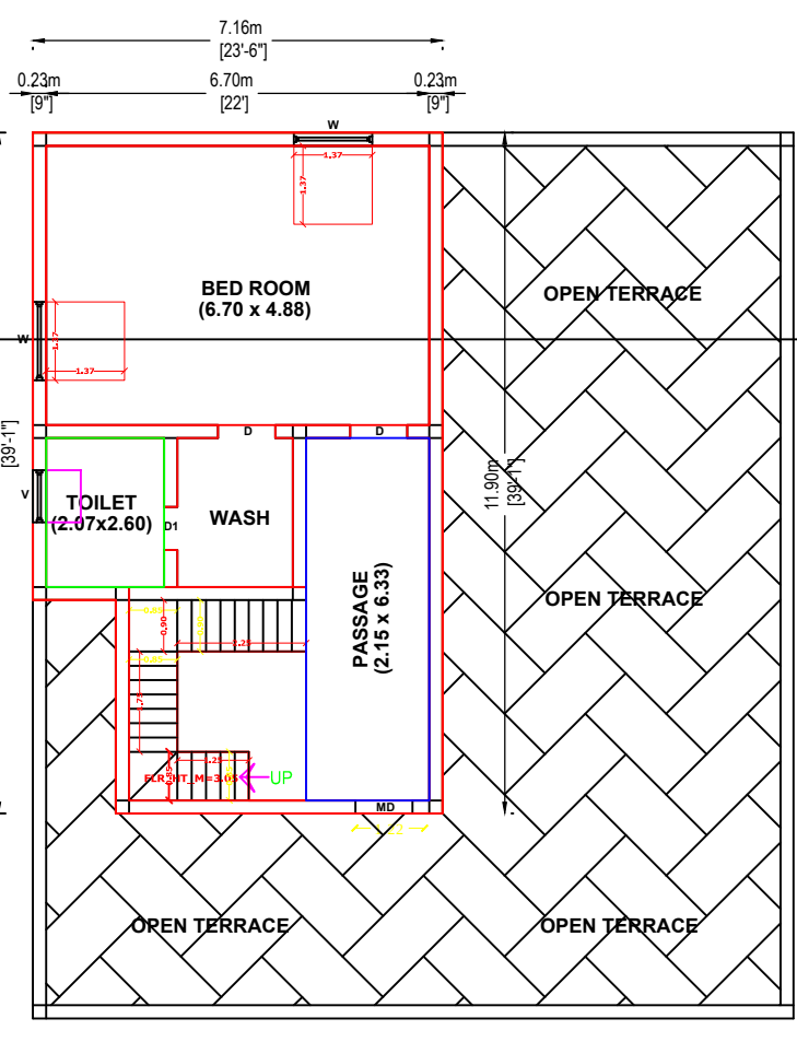
FIRST FLOOR BUILDING PLAN
