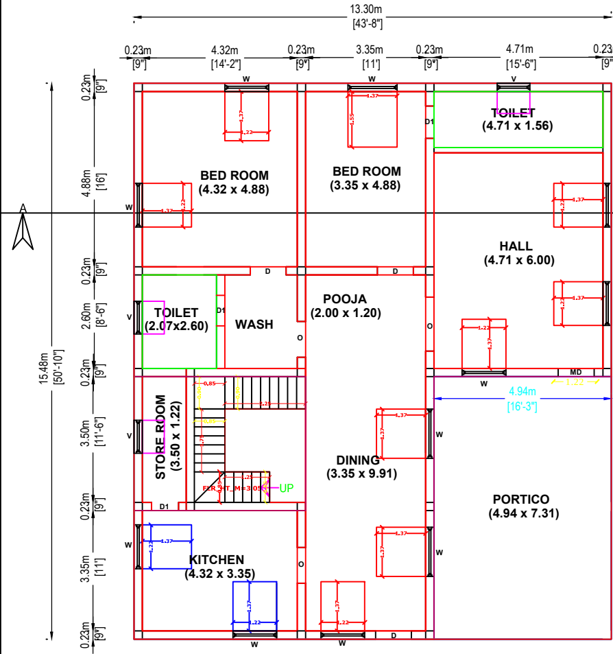
GROUND FLOOR BUILDING PLAN
