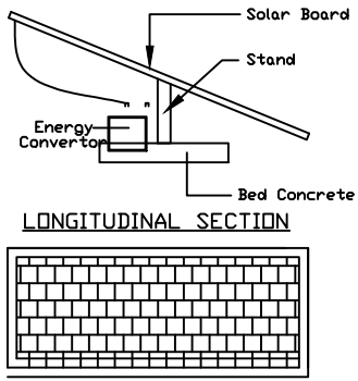
PLAN SOLAR SYSTEM Not To Scale
