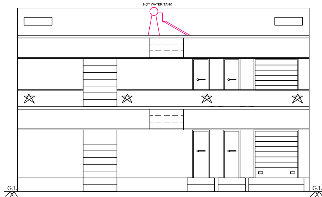
FRONT ELEVATION [EAST SIDE]
