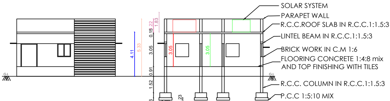
ELEVATION FACING ON WEST
