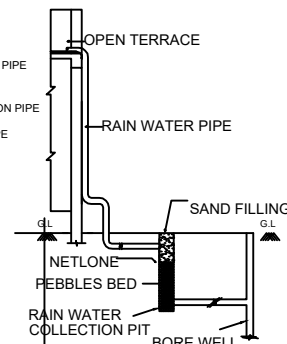
RAIN WATER
