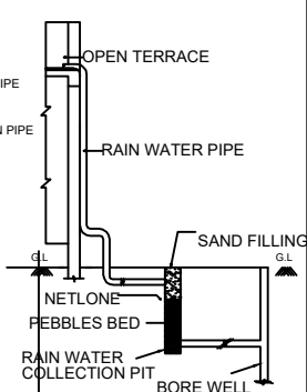
RAIN WATER
