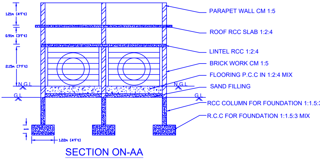
SECTION ON-AA
