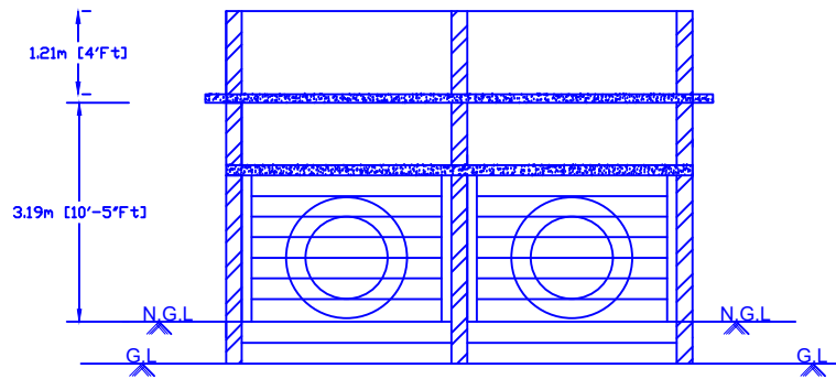
ELEVATION SOUTH FACING
