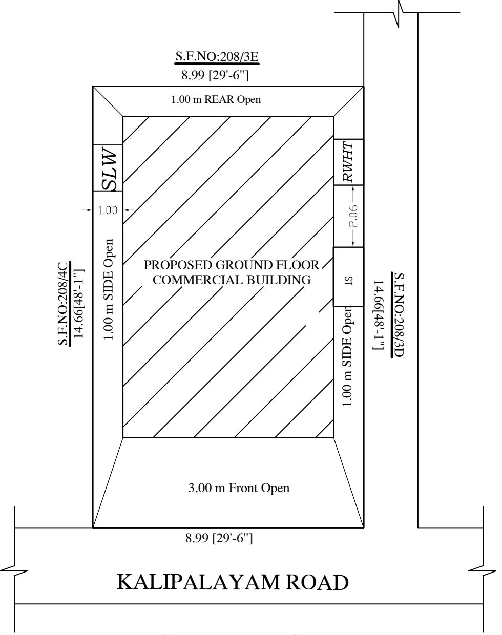
SITE LAYOUT
