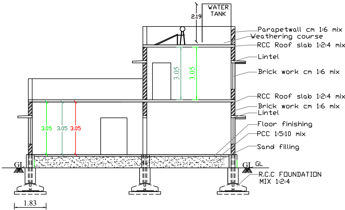
SECTION 'AA'
