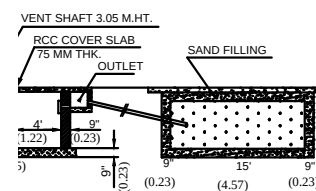
ON SEPTIC TANK & DISP-TRENCH
