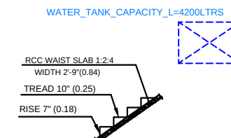
STAIRCASE DETAIL SCALE 1:50
