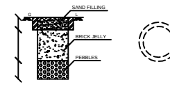
RAIN WATER HARVESTING SYSTEM SCALE 1:50
