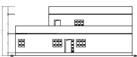
ELEVATION FACING NORTH
