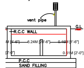
SECTION ON D-D
