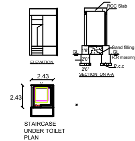
STAIRCASE UNDER TOILET PLAN
