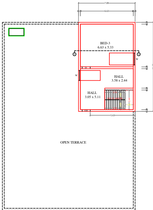
FLOOR-1
