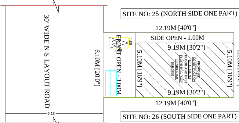
SITE PLAN
