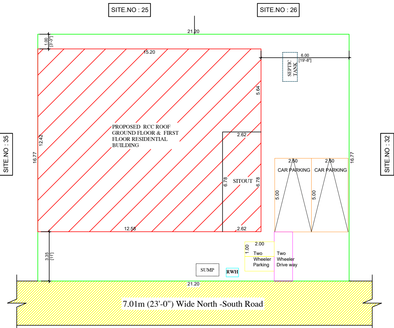
SITE PLAN
