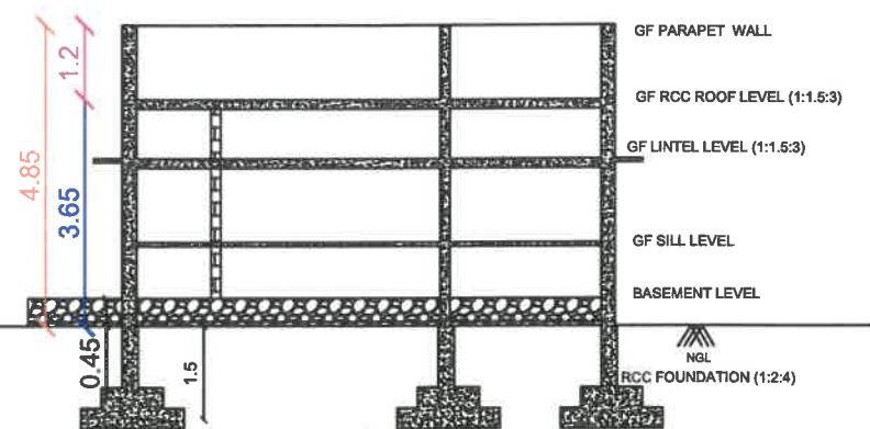
SECTIONAL VIEW ON A-A
