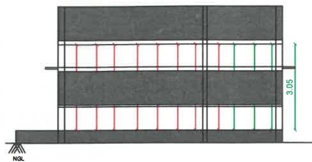
SOUTH ELEVATION
