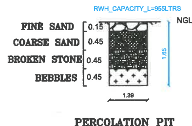
PERCOLATION PIT
