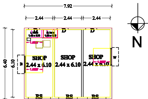
G.F.SHOP PLAN
