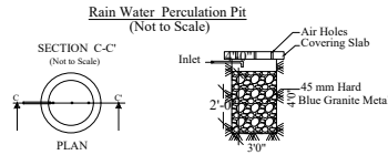
Rain Water Percolation Pit
