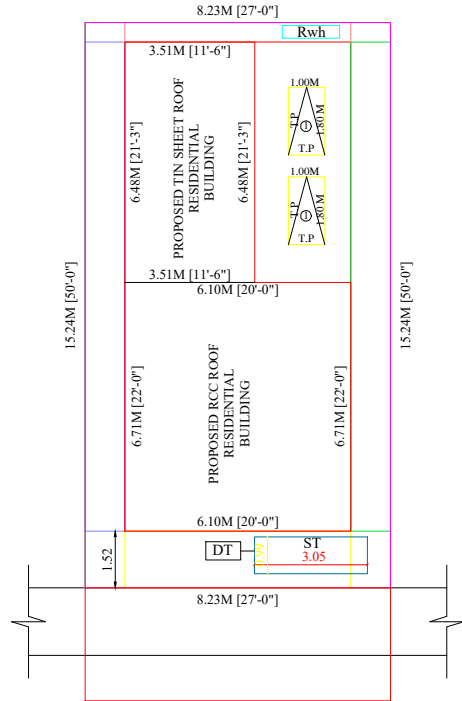
SITE PLAN (MEANT FOR CONSTRUCTION)
