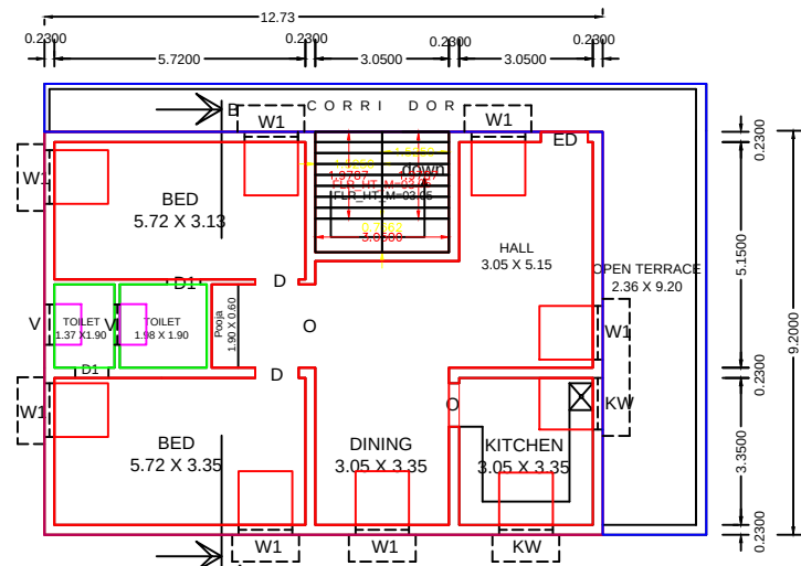
PROPOSED FIRST FLOOR PLAN [SCALE 1:100]
