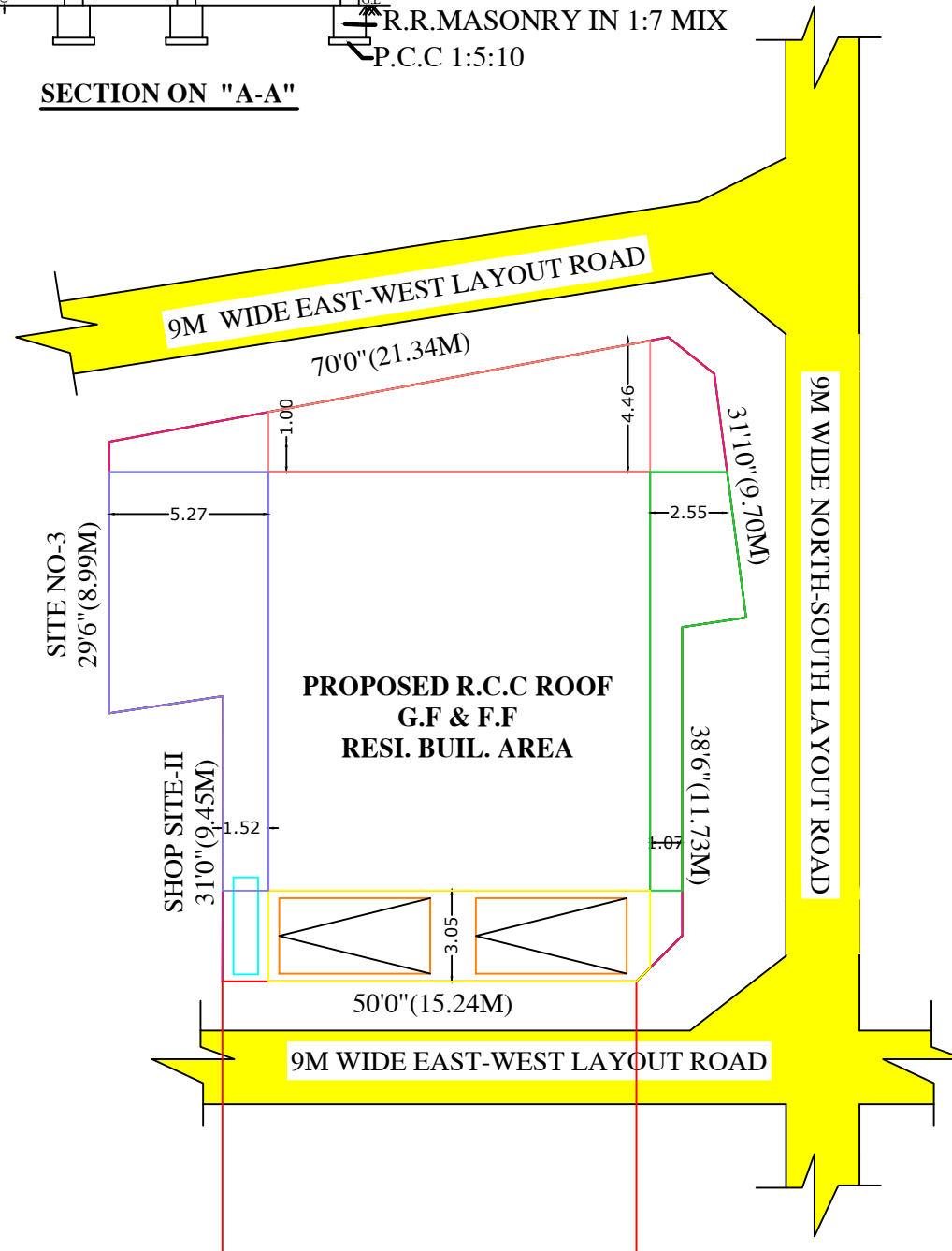
SITE PLAN
