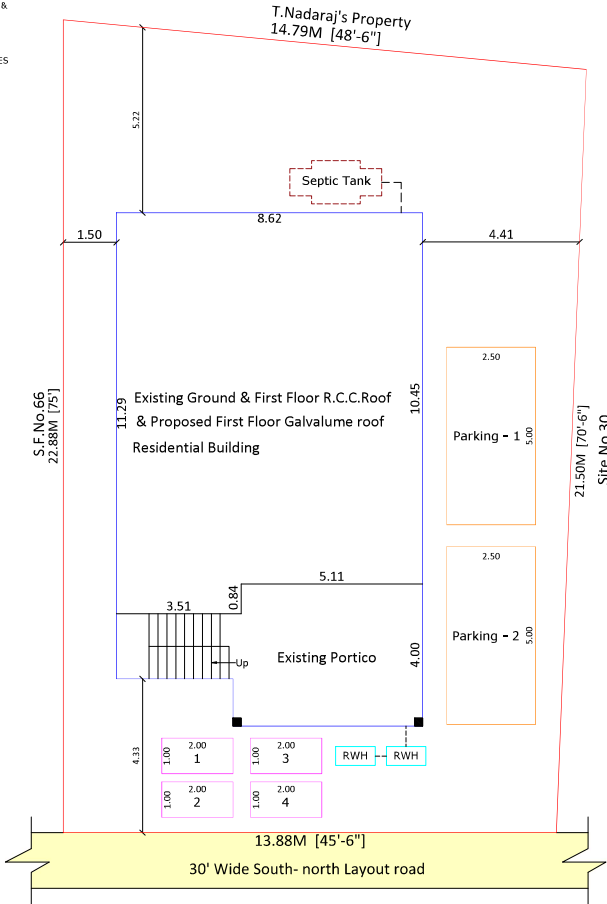
SITE PLAN
