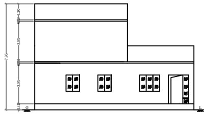
ELEVATION FACING EAST
