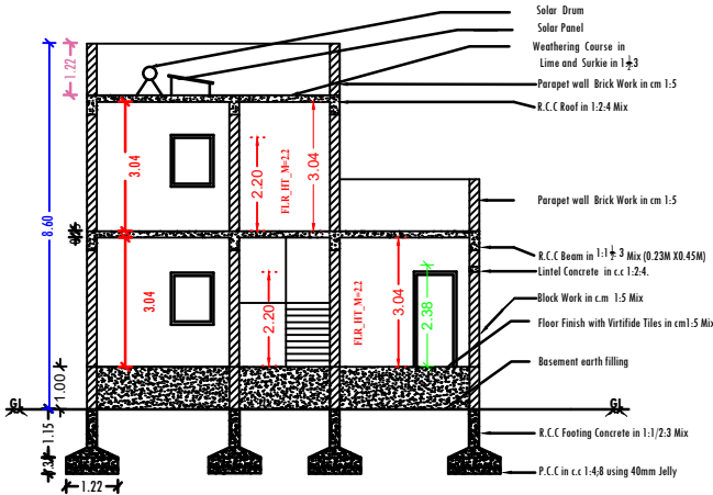
Section on "BC"
