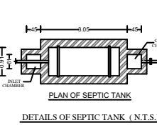
PLAN OF SEPTIC TANK
