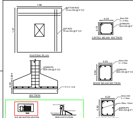
COLUMN SECTION
