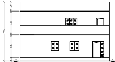
ELEVATION FACING EAST
