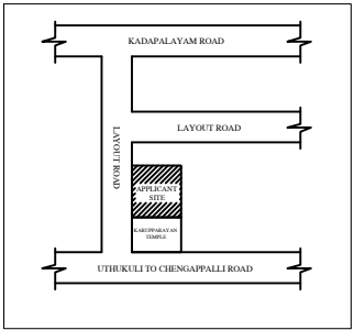
KEY PLAN 1:10000
