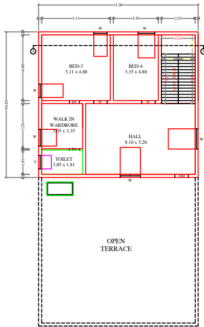
FLOOR - 1
