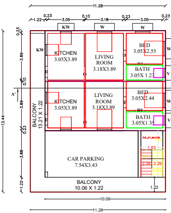
GROUND FLOOR FACING EAST
