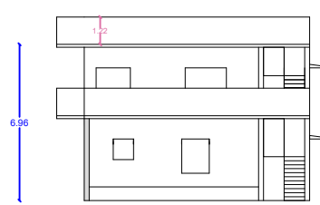
ELEVATION FACING EAST
